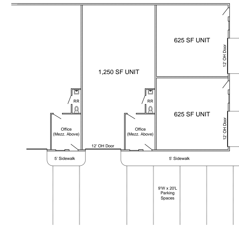
Building Detail Scale: 1/16"=1'
